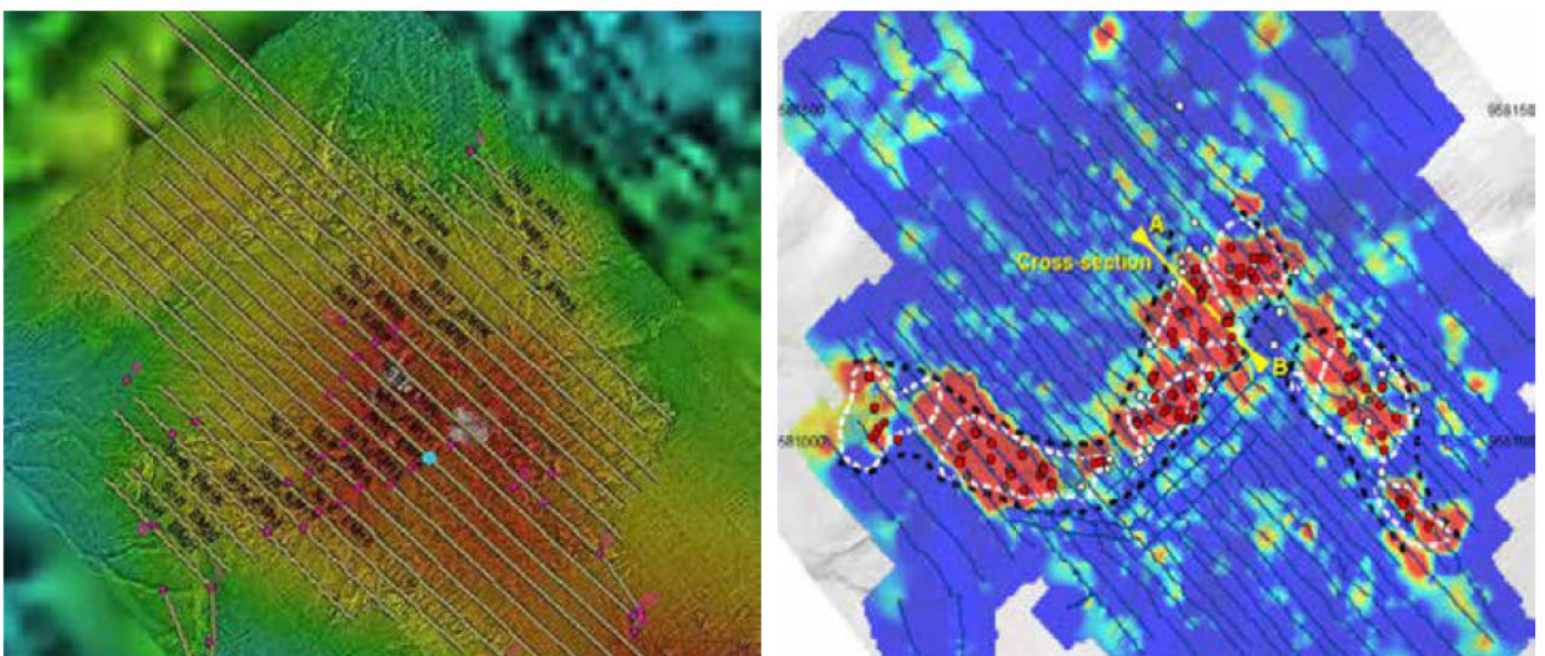
EM survey of Nautilus' Solwara 1 seafloor massive sulphide deposit
