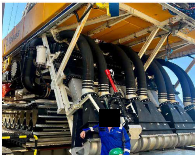
Below: Robert Heydon with the seafloor collector used in the NORI polymetallic nodule trial harvesting
