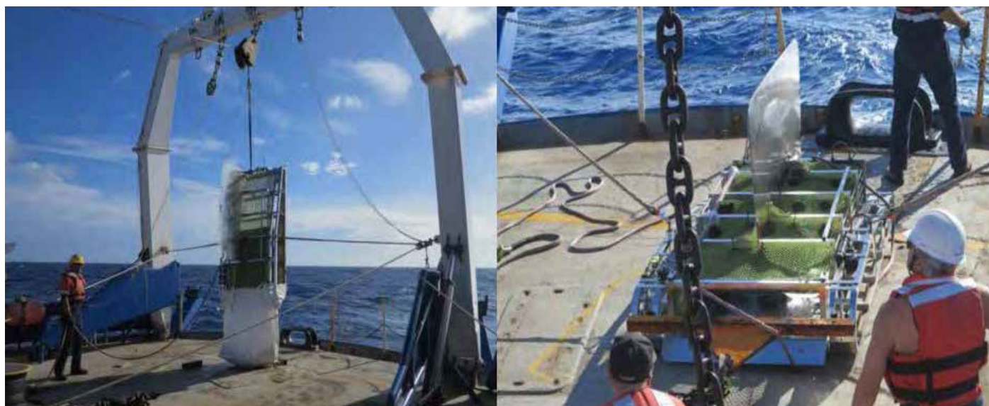
Above: The epibenthic sled used to collect nodules during the 2013 NORI Cruise Below: Polymetallic nodules recovered during the 2013 NORI Cruise Source: Technical Report Summary, AMC Project 321012, 17 March 2021
